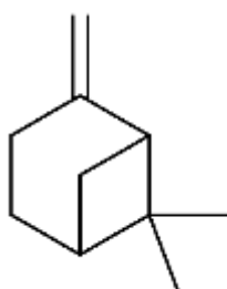
Beta-pinene
